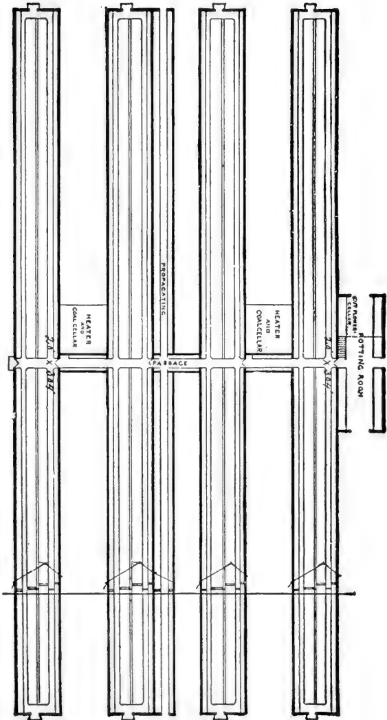
FIG. 79. GROUND PLAN OF F. R. PIERSON'S RANGE.
